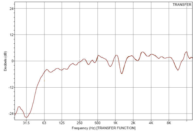
Radian 12" with 60 deg horn
