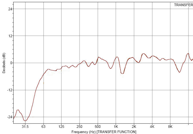
Radian 12" with 90 deg horn
