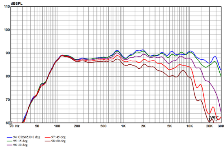
Directivity response curves of CRS6530 with recommended XO in V_b=6.5 L/ F_b=65 Hz vented box, free field.
