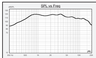
Amplitude vs. Frequency of the Radian 651PB measured on a 2" (50.8mm) high frequency horn with a one watt (2.83 Vrms) input at 8 ohms.
