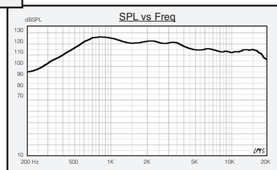
Amplitude vs. Frequency of the Radian 760PB measured on a 2" (50.8mm) high frequency; horn with a one watt (2.83 Vrms) input at 8 ohms.
