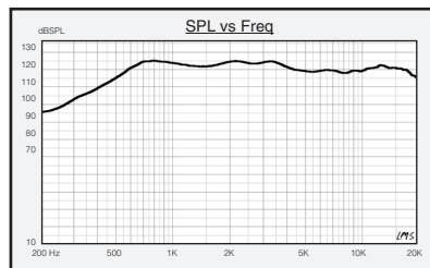
Amplitude vs. Frequency of the Radian 760PB measured on a 2" (50.8mm) high frequency; horn with a one watt (2.83 Vrms) input at 8 ohms.
