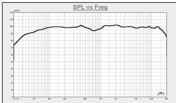
Amplitude vs. Frequency Response of the Radian 1512NEO as measured on axis with a one watt (2.83 Vrms), swept sine wave input at 8 ohms, using a 322/15 crossover network in a 3.4 (ft. 3 ) vented cabinet.
