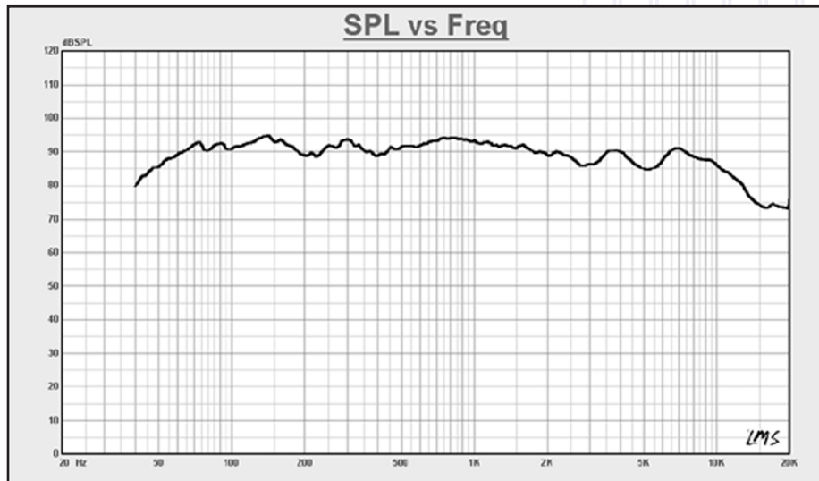
Amplitude vs. Frequency of the Radian 365 as measured on axis with a one watt (2.03 Vrms), swept sine wave input at 4 ohms.
